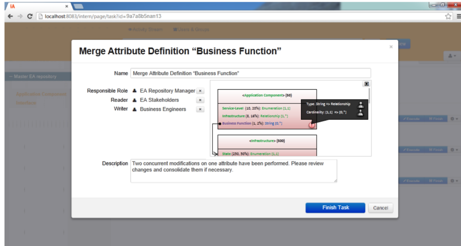
Fig. 5. Automatically generated merge task after the update/update model conflict
