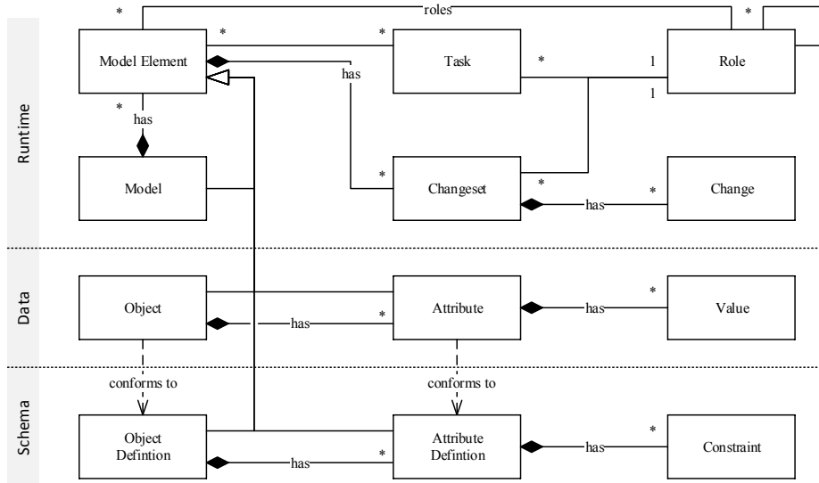
Fig. 2. A meta-information model facilitating model evolution at runtime
