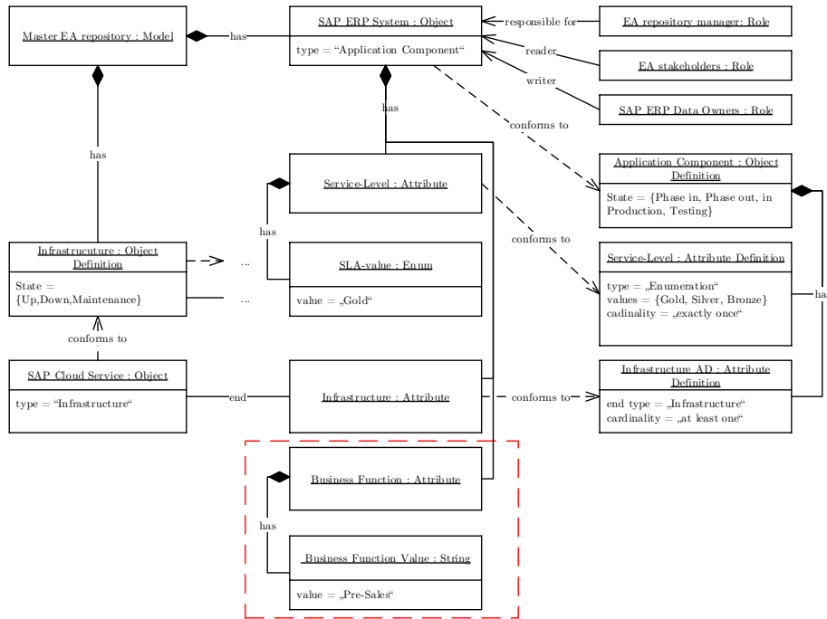
Fig. 3. Adapted EA information model containing a new business function
