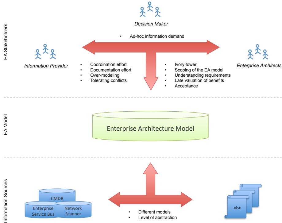
Fig. 1. Challenges for EA modeling and documentation at runtime
