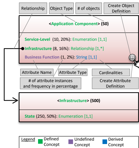
Fig. 4. Graphical representation of the EA information model
