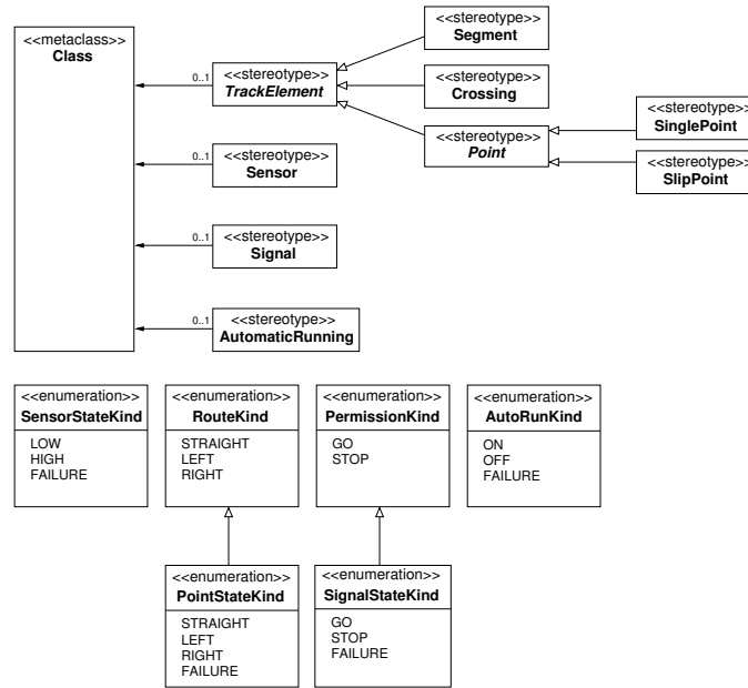
Fig. 2. Network elements of the RCSD profile
