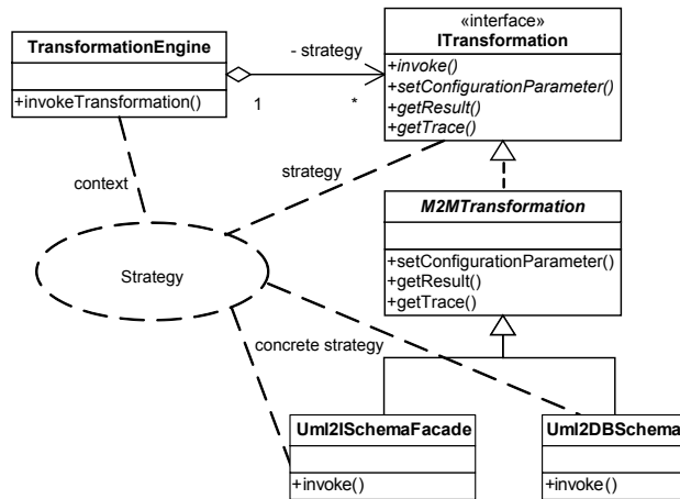
Fig. 1. Architecture of the Transformation Framework
